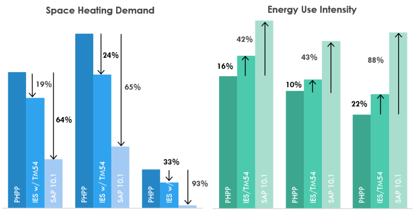
Figure 2 Software modelling comparisons for three buildings
