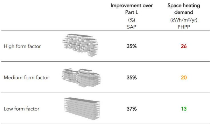
Figure 1 Illustration of how similar SAP performance varies in real life 11
