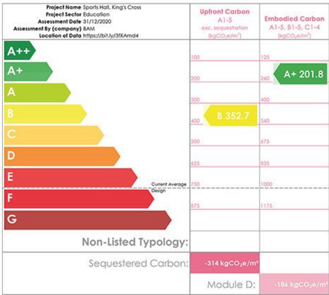
Figure 5 Emondiied carbon reporting example, Bennetts Associates 30
